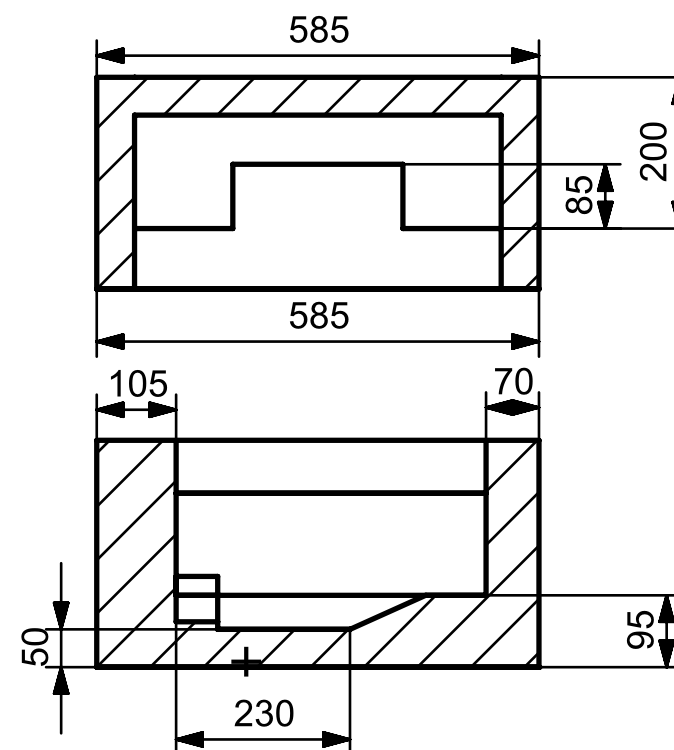
SECTION E-E
