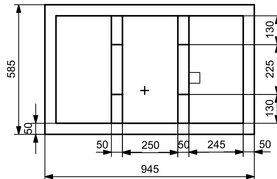
SECTION E-E
